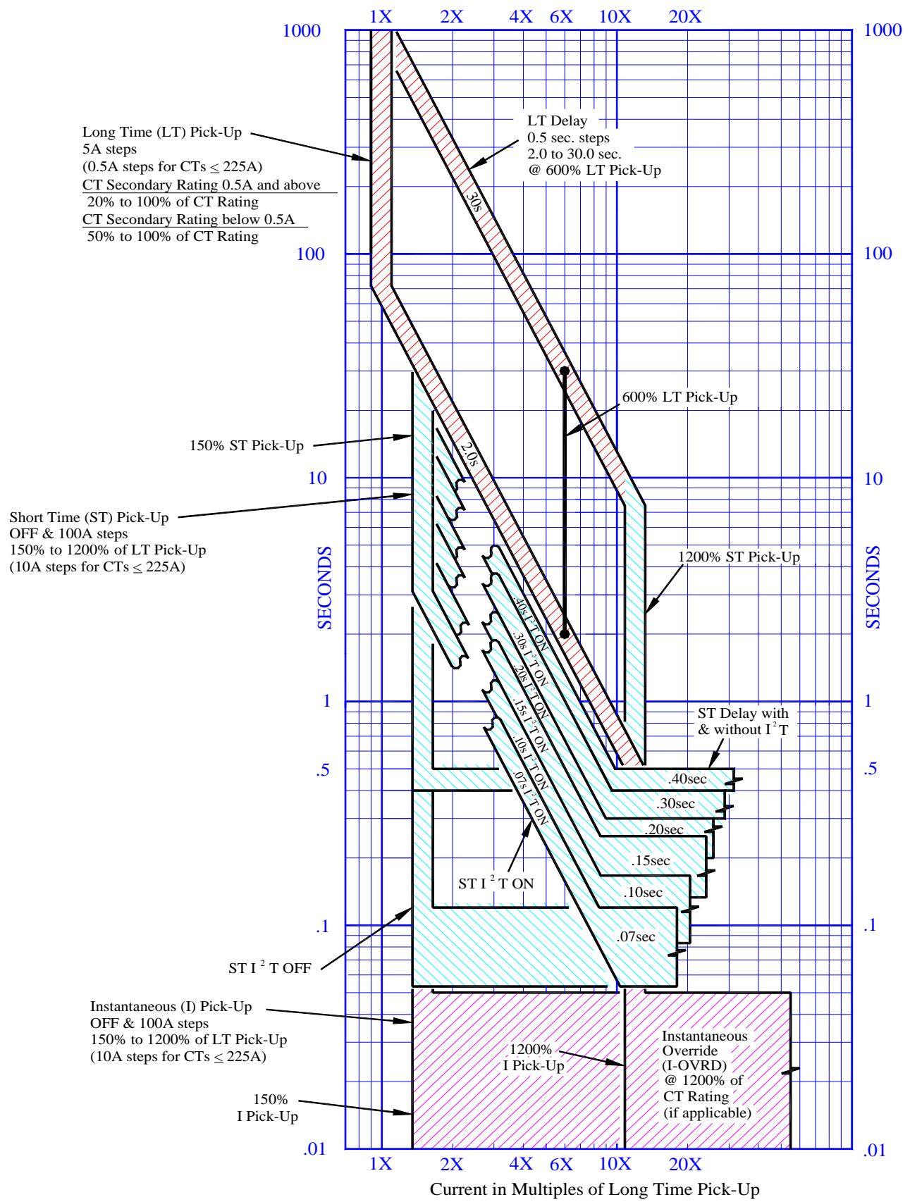
Figure 12: AC-PRO-II Overload TCC
