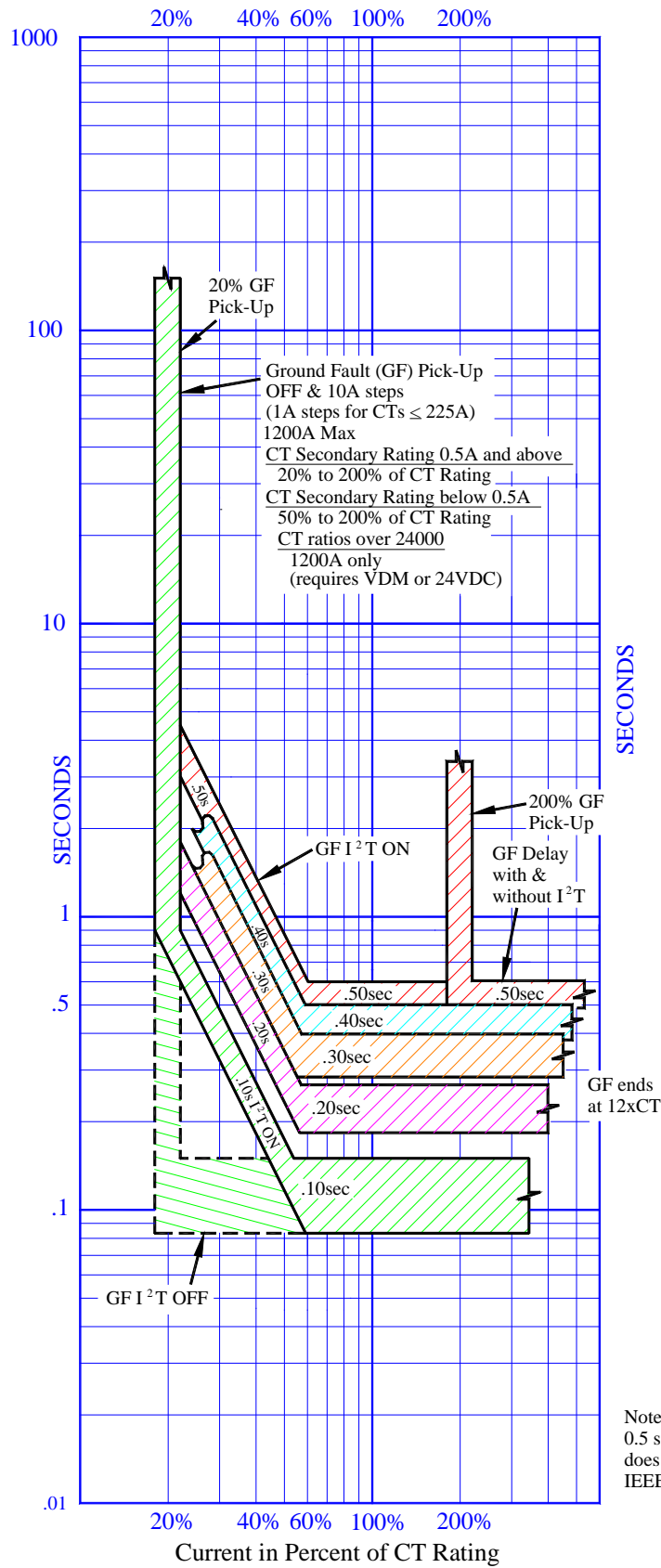
Figure 13: AC-PRO-II Ground Fault TCC
