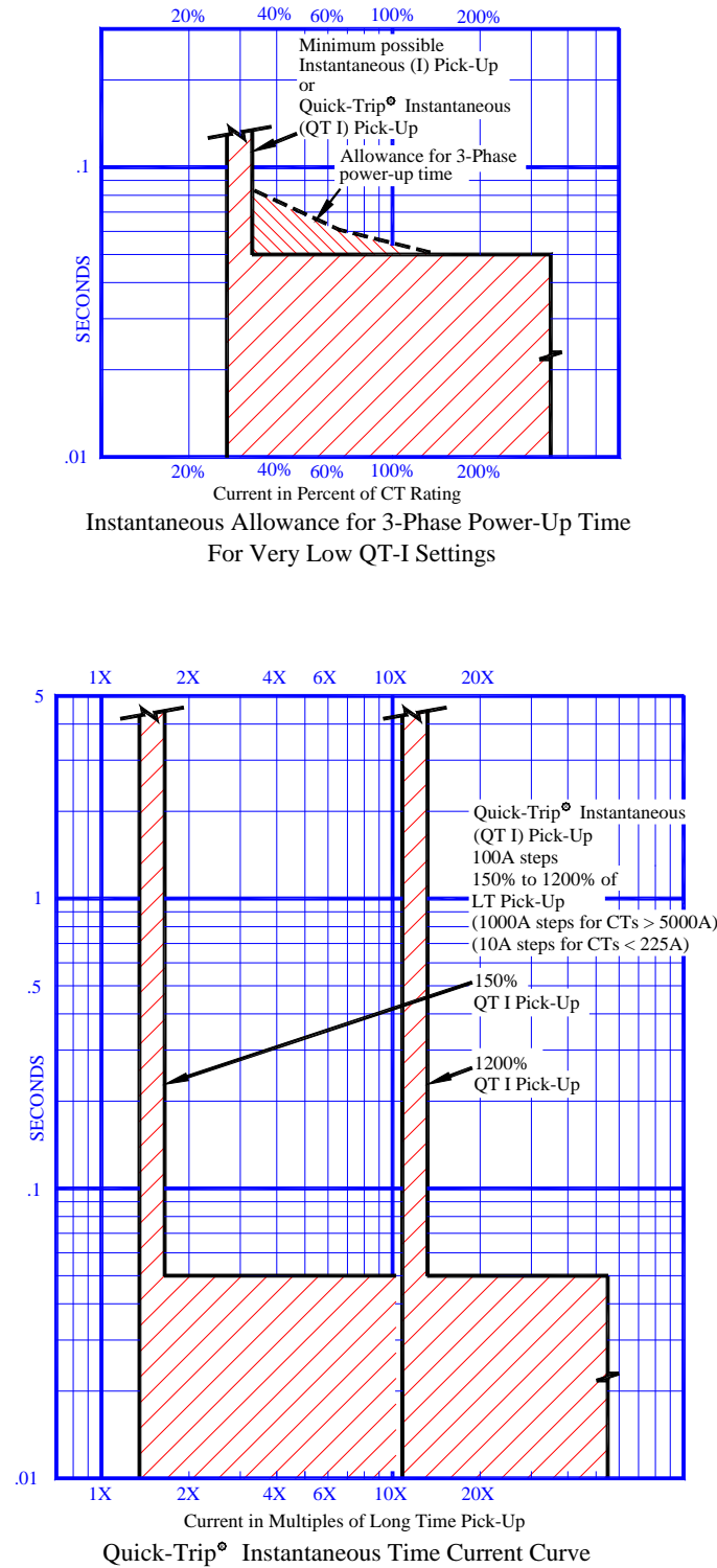
Figure 11: AC-PRO Quick-Trip TCC
